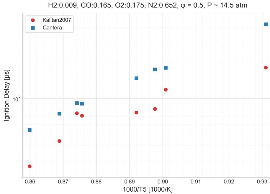
Figure 4.13: Comparison of Cantera IDT simulation with experimental measurement good_cantera IDT Type: d(OH * )/dt max.
