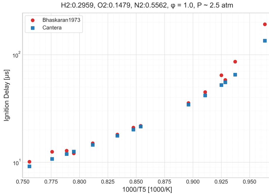
Figure 4.12: Comparison of Cantera IDT simulation with experimental measurement asda IDT Type: dP/dt max.
